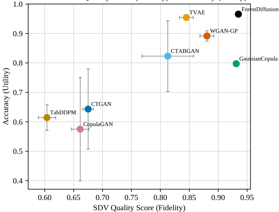
Cancer: SDV Quality Score (Fidelity) vs Accuracy (Utility)
